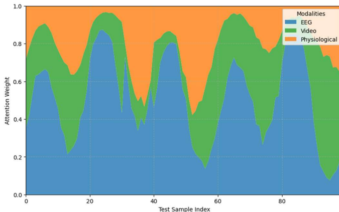
Figure 3. Dynamic contribution of EEG, video, and physiological modalities to the final decision across varying diagnostic scenarios
